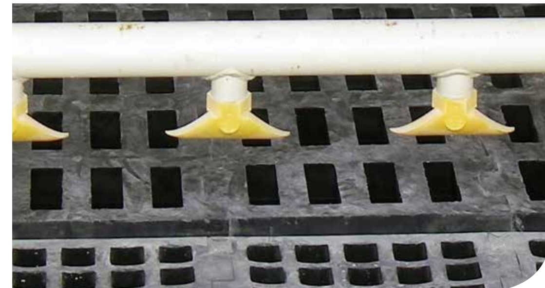
HiPer Life modules on FS-screen in feed end to handle impact with better life time.
