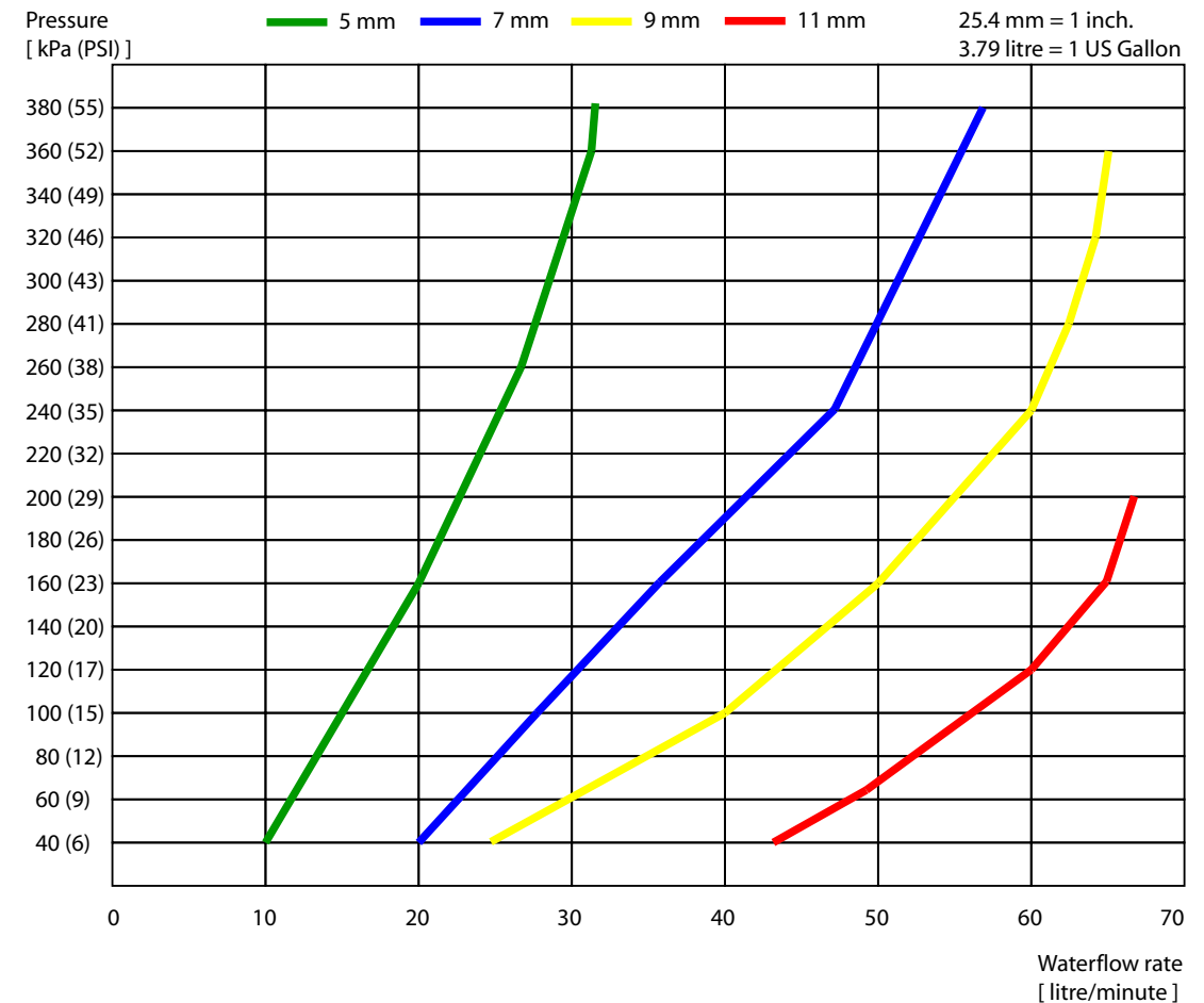
Water flow rate in relation to pressure
