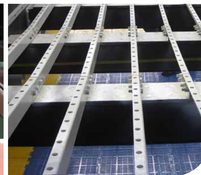
LS-PS rails on mining screen
